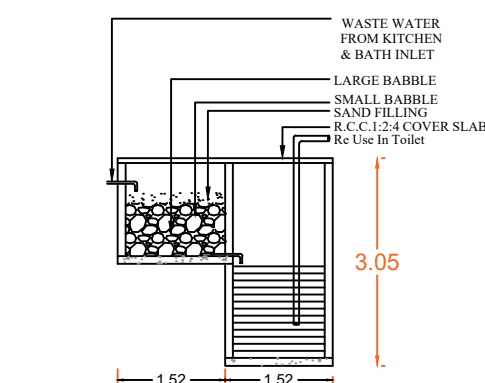
RECYCLING OF WASTE WATER FROM KITCHEN & BATHROOM NOT IN SCALE
