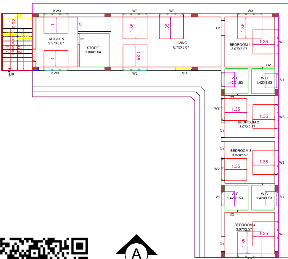
D FLOOR SCALE 1:100
