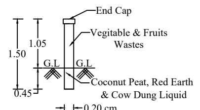
PIPE COMPOSTER
