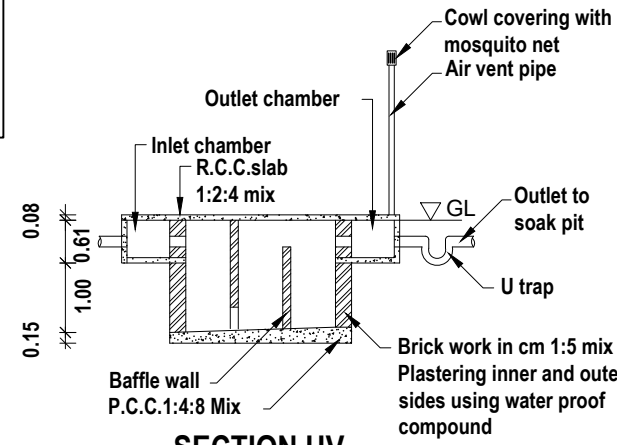
SECTION UV
