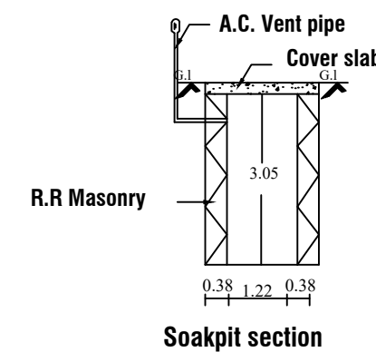
Soakpit section
