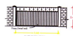
GATE ELEVATION
