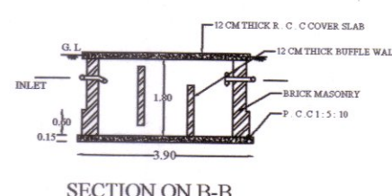
SECTION ON B-B
