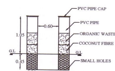
PIPE COMPOSIT PIT
