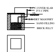
RAIN WATER HARVEST ARRANGEMENTS
