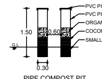
PIPE COMPOST PIT
