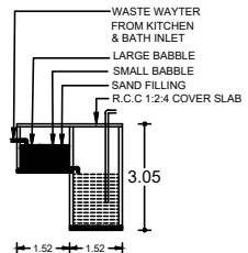
RECYCLING OF WASTE WATER TANK
