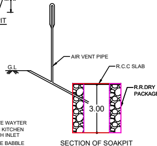
SECTION OF SOAKPIT
