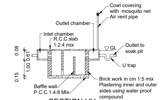
SECTION UVV
