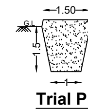
Trial Pit
