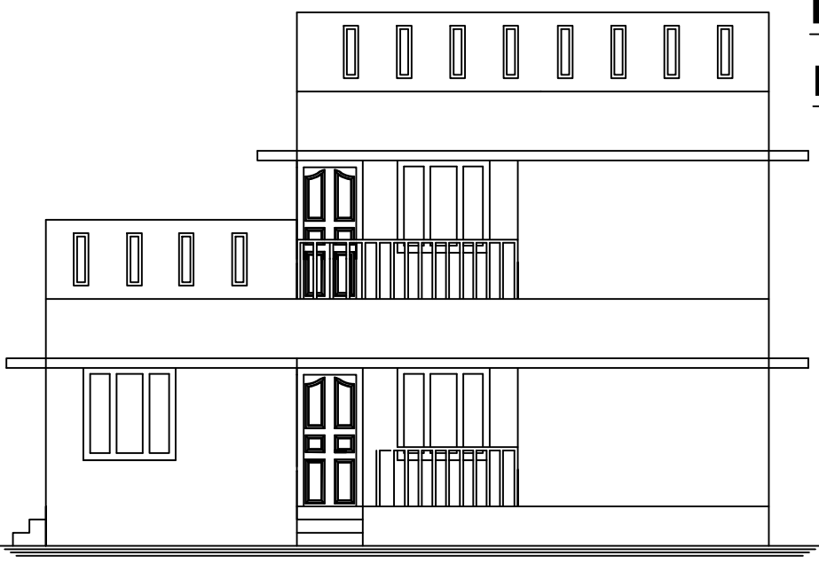
FRONT ELEVATION
