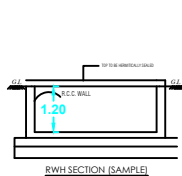
RWH SECTION (SAMPLE)
