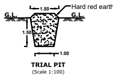
TRIAL PIT (Scale 1:100)
