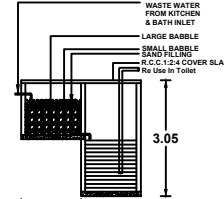
RECYCLING OF WASTE WATER FROM KITCHEN & BATHROOM
