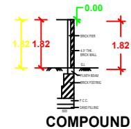
COMPOUND WALL
