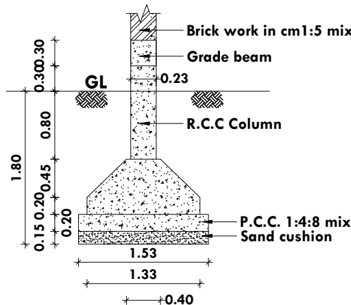
COLUMN DETAILS DETAIL "A" SCALE 1:50
