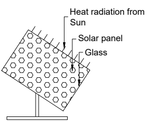
SOLAR SYSTEM
