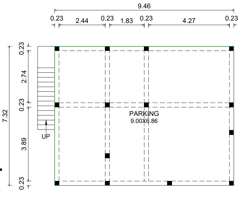
CELLAR FLOOR PLAN
