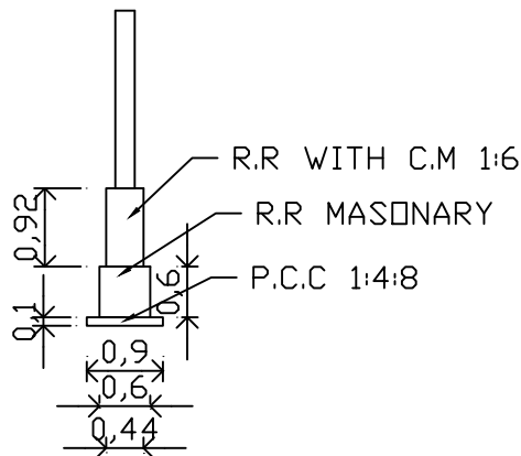
FOUNDATION
