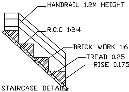
STAIRCASE DETAIL
