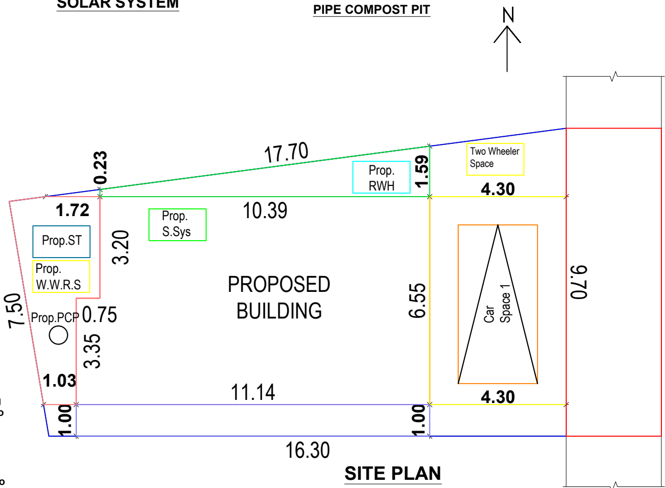
SOLAR SYSTEM
