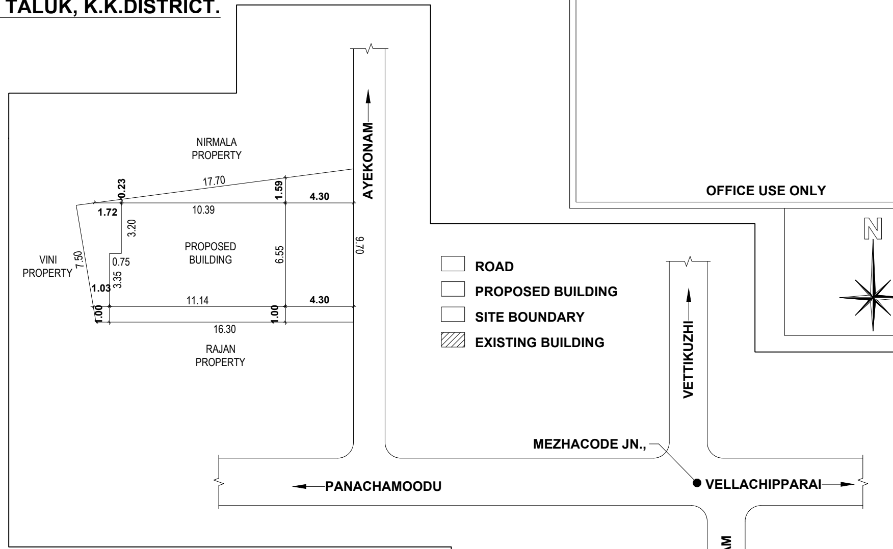
KEY PLAN SCALE:1:400.
