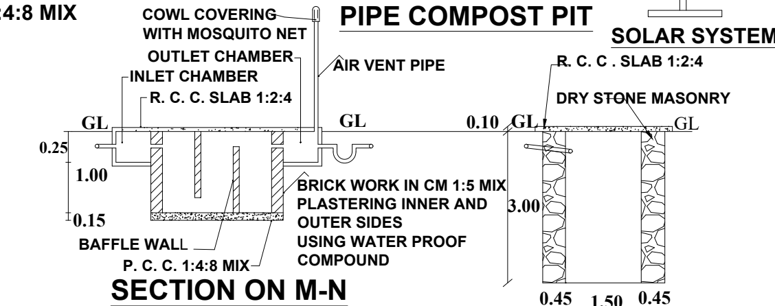
SECTION ON M-N
