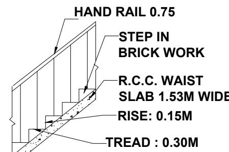
STAIR DETAIL
