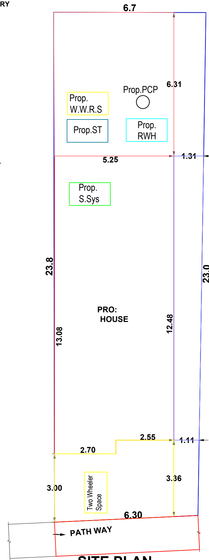
SITE PLAN
