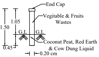
PIPE COMPOSTER
