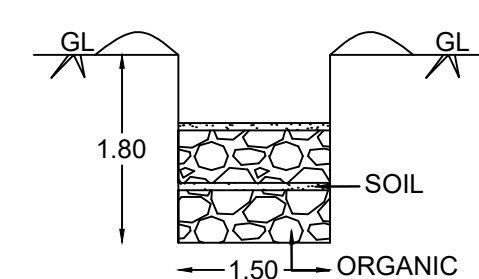
COMPOST PIT
