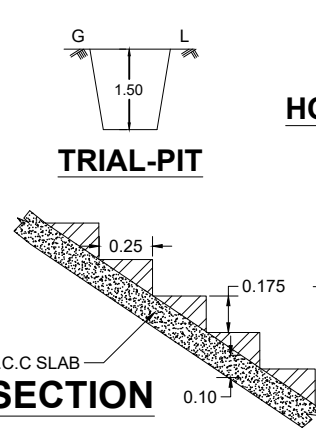
SECTION ON BB
