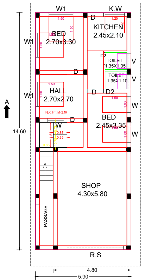
G.F. PLAN
