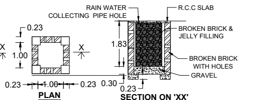
RAIN WATER HARVEST WELL
