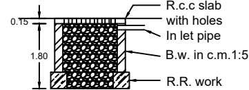
R.C.C. slab with holes In let pipe B.w. in c.m.1:5 R.R. work
