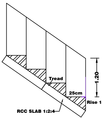
STAIR DETAILS
