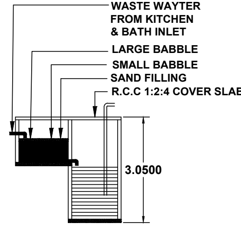
RECYCLING OF WASTE WATER TANK
