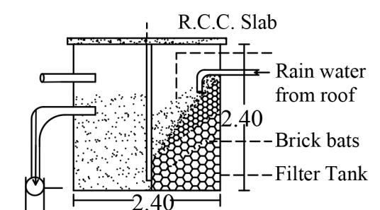
Rain Water Storage RWH_CAPACITY_L=4800LTRS
