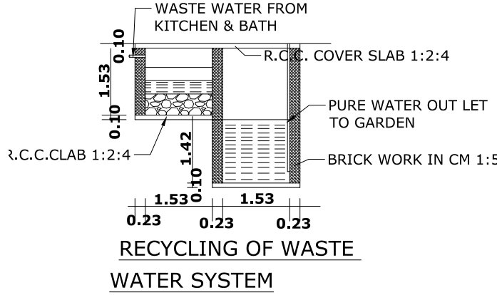
RECYCLING OF WASTE WATER SYSTEM
