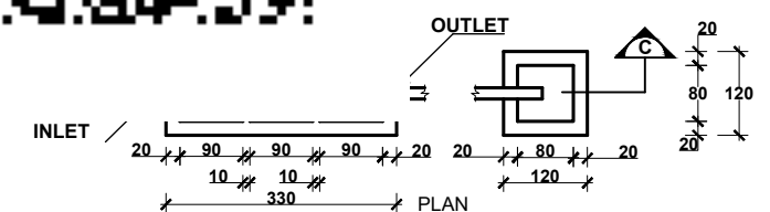
WASTE WATER PIT
