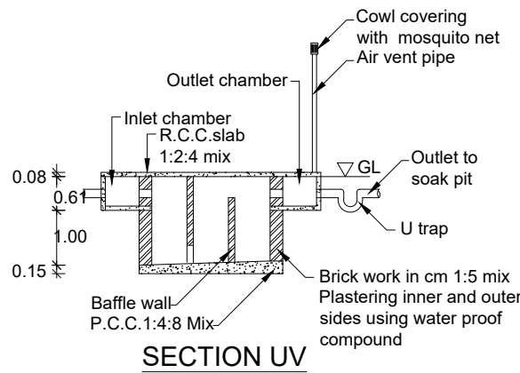
SECTION UV
