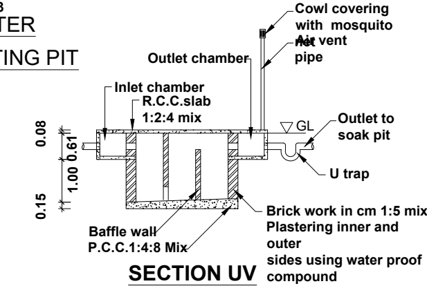
SECTION UV
