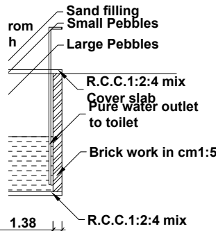
WASTE WATER RECYCLING SYSTEM
