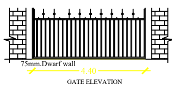
GATE ELEVATION
