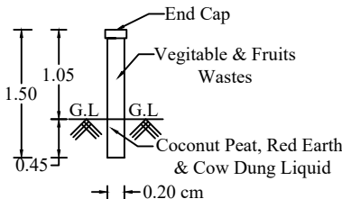
PIPE COMPOSTER
