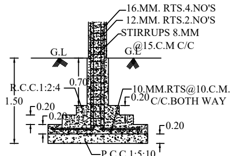
COLUMN SECTION
