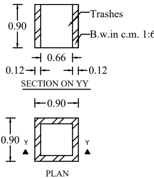
WASTE TRASH PIT
