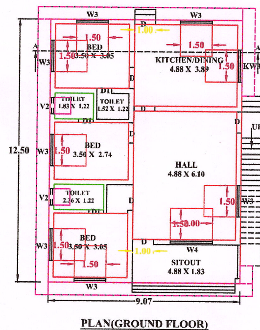
PLAN(GROUND FLOOR)
