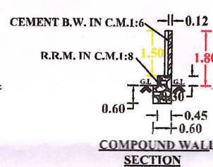
COMPOUND WALL SECTION
