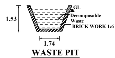
WASTE PIT
