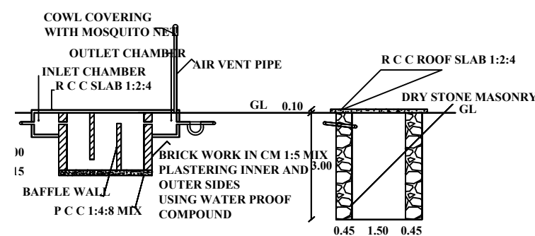
SECTION ON M-N
