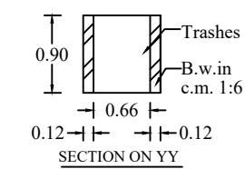
SECTION ON YY
