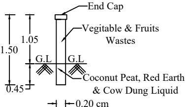
PIPE COMPOSTER
