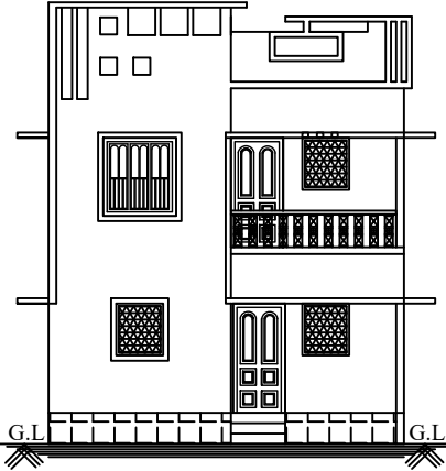
FRONT ELEVATION
