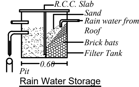
Rain Water Storage
