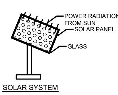
SOLAR SYSTEM
