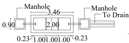
SECTION DETAILS OF SEPTIC TANK
