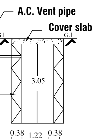
Soakpit section
