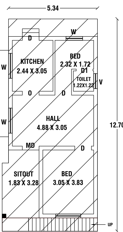
GROUND FLOOR PLAN SCALE 1:100 ALL DIMENSIONS ARE IN METER
