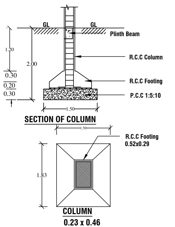
SECTION OF COLUMN
