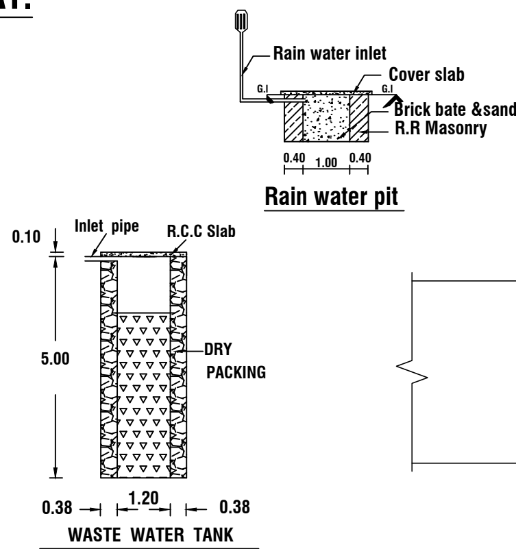
RAIN WATER PIT
