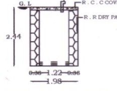
RAIN WATER STORAGE TANK SECTION
