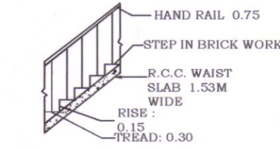
STAIR CASE SECTION
