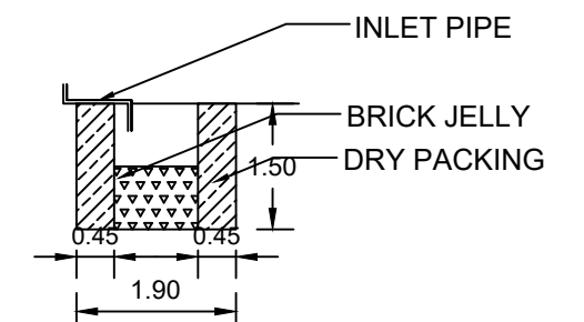
RAINWATER HARVESTING
