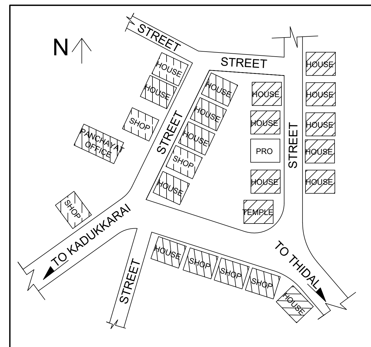
KEY PLAN
