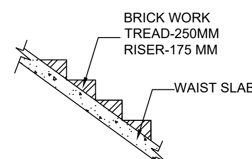
STAIRCASE DETAILS
