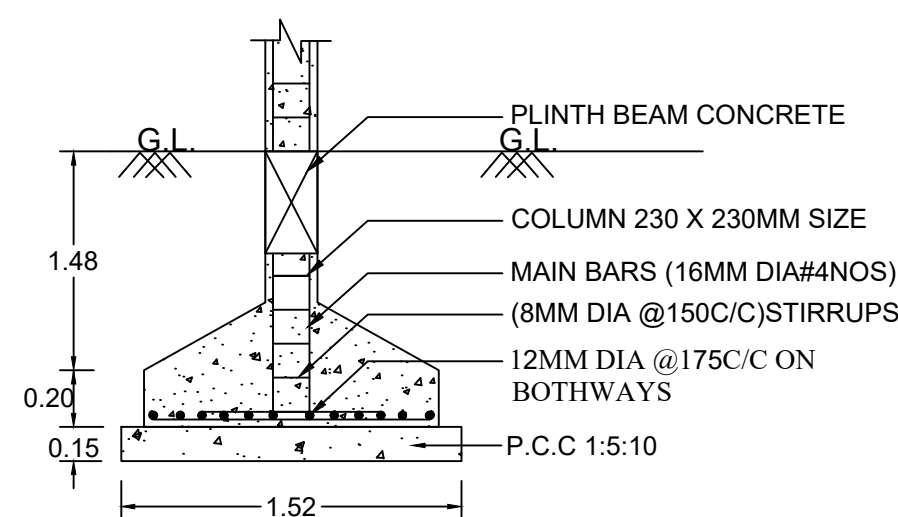
COLUMN FOOTING
