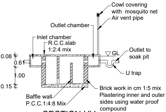
SECTION UV
