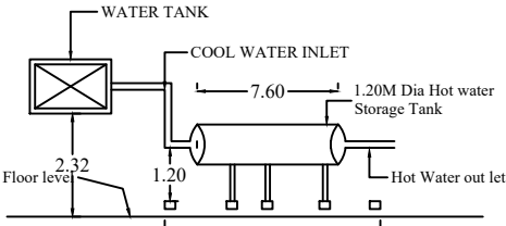
SOLAR WATER HEATING SYSTEM (S.W.H.S.DETAILS)
