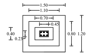
COLUMN PLAN (0.38x0.23 Size)
