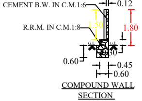
COMPOUND WALL SECTION
