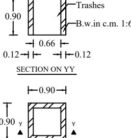
WASTE TRASH PIT
