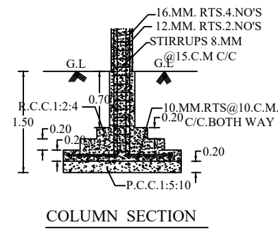
COLUMN SECTION
