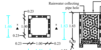
RAIN WATER HARVEST WELL
