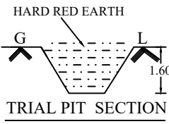
TRIAL PIT SECTION
