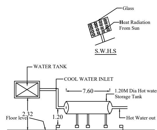
SOLAR WATER HEATING SYSTEM (S.W.H.S.DETAILS)
