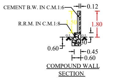
COMPOUND WALL SECTION
