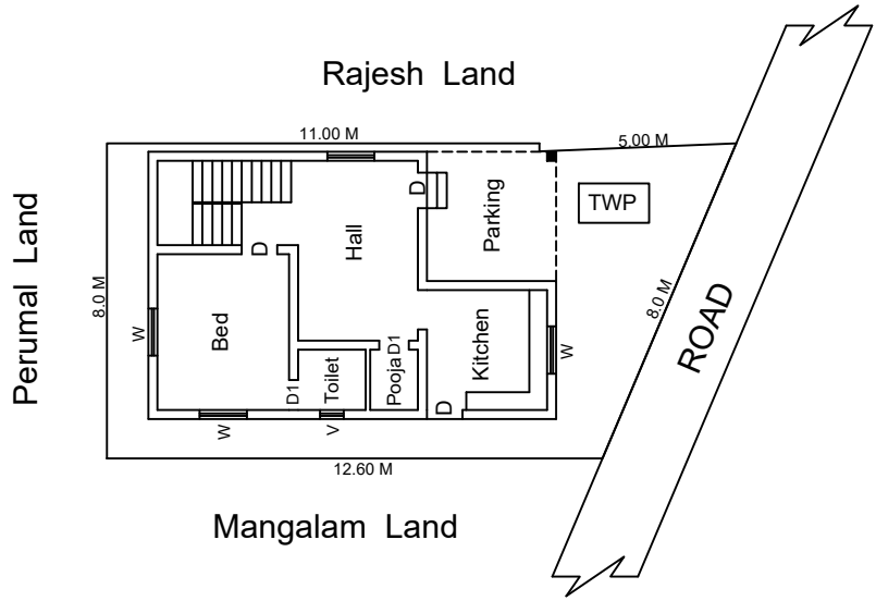
SITE PLAN
