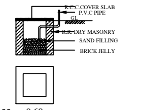
RAIN WATER HARVEST ARRANGEMENTS
