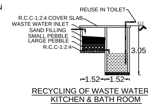
RECYCLING OF WASTE WATER KITCHEN & BATH ROOM
