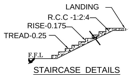
STAIRCASE DETAILS
