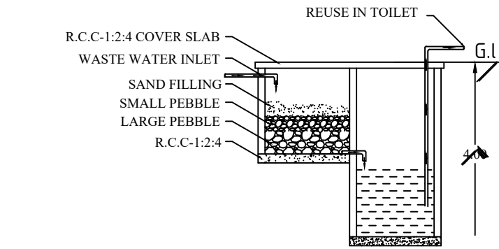
RECYCLING OF WASTE WATER KITCHEN & BATH ROOM
