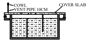
SECTION OF SEPTIC TANK
