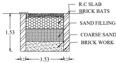
RAIN WATER HARVESTING TANK
