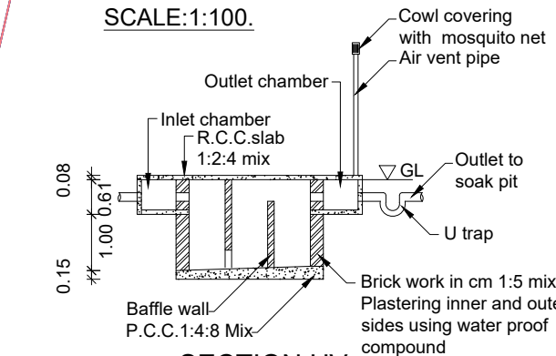
SECTION UV
