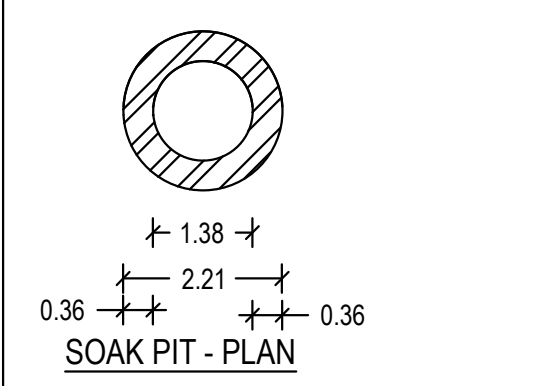
SOAK PIT - PLAN
