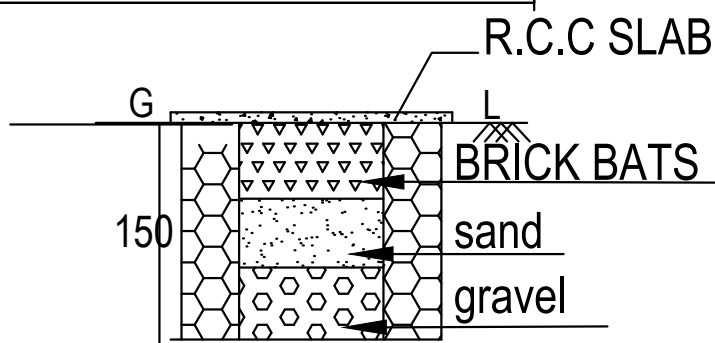
RWH TANK
