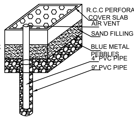
PERCOLATION BORE PIT
