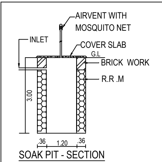
SOAK PIT - SECTION
