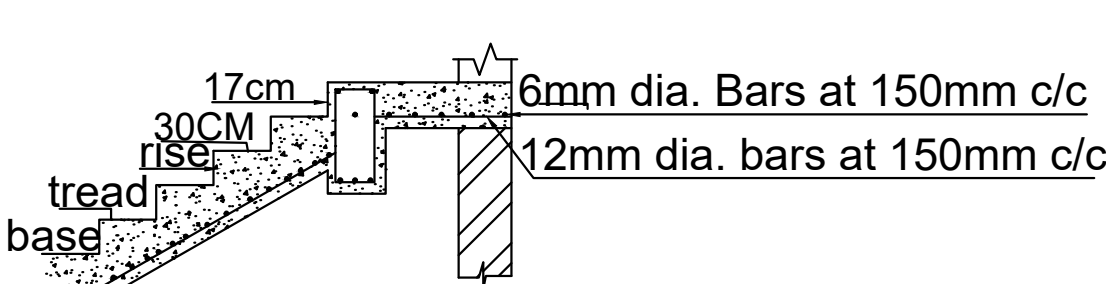
SECTION OF STAIRCASE
