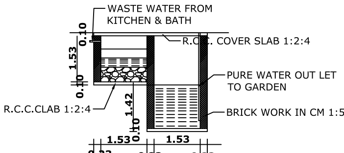
RECYCLING OF WASTE WATER SYSTEM
