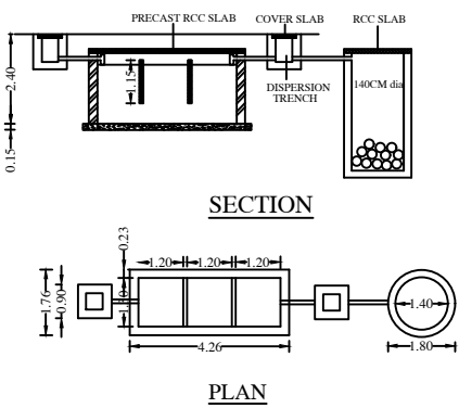
SEPTIC TANK
